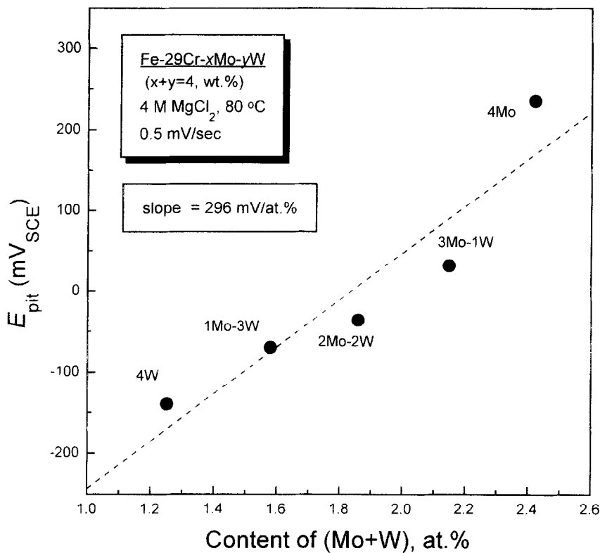
Fig. 5. Dependence of E_{\text{pit}} on (Mo + W) at% for Fe-29Cr ferritic stainless steels in 4 M \text{MgCl}_2 solution at 80 °C.
